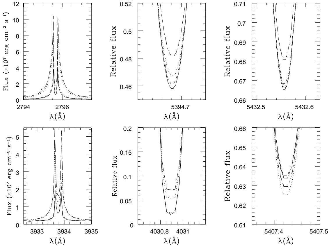
Fig. 3. Top row from left to right - line profiles Mg II k with Mn I (uv1), Mn I 5395Å (1) and 5432Å (1). Bottom row — line profiles for Ca II K 3933Å, Mn I 4031Å (2) and Mn I 5407Å (4). Profiles shown are for atmospheres with (\log m_0, \log m_{\text{TR}}) = (-2.5, -5.0) full line, (-2.5, -4.6) dashed line, (-1.5, -5.0) dotted line and (-1.5, -4.6) long-dashed line
