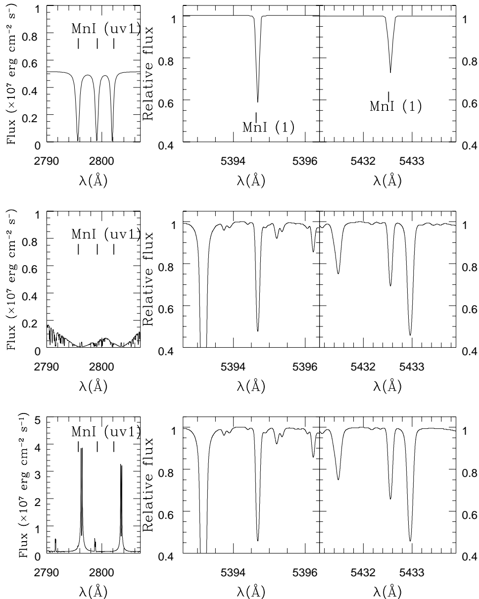
Fig. 4. The top two panels show the results of NLTE calculation for Mn I without any interaction with Mg II and no line blanketing. In the middle row, we show the results of NLTE Mn I obtained with Mg II LTE line opacities included (but not treated explicitly as a line transfer) and bottom row the results when both Mn I and Mg II are treated in NLTE. The atmosphere has \log m_0 = -2.5 and \log m_{\text{TR}} = -5.0
