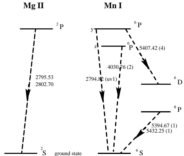
Fig. 2. A partial term diagram of Mg II and Mn I for the lines used in this study.
